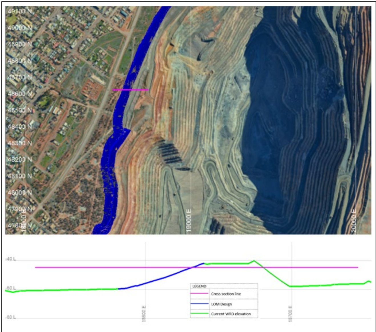
Figure 9-21: Fimiston Noise Bund WRD Closure Design and Cross Section
