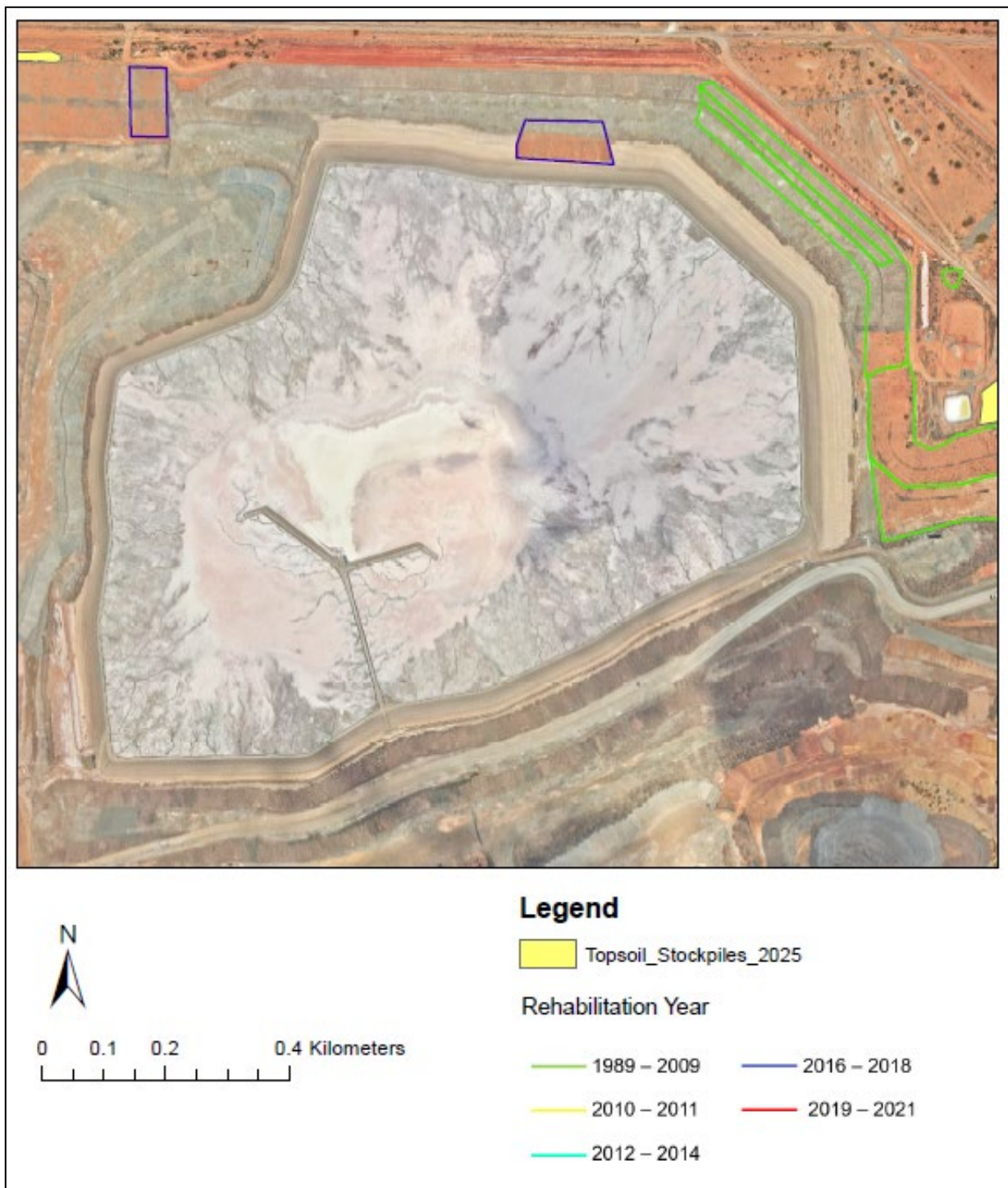
Figure 9-27: Fimiston I TSF current rehabilitation status (2025)
