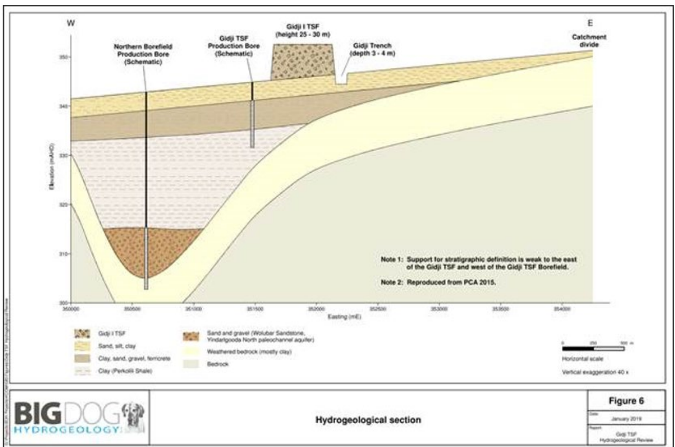
Figure 9-9-45: East-West Hydrogeological Section at Gidji
