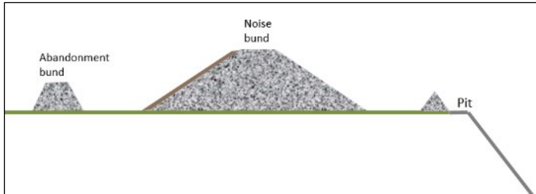
Figure 9-8: Option A: Western abandonment bund located separate from the Noise Bund
