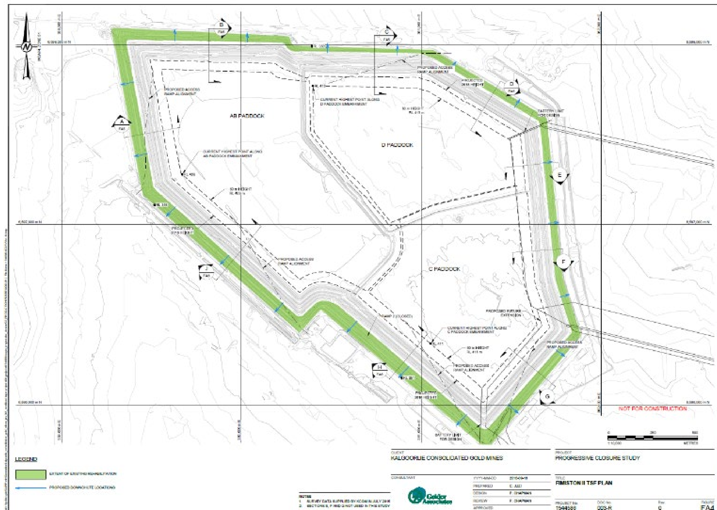
Figure 9-32: Fimiston II TSF Closure Design
