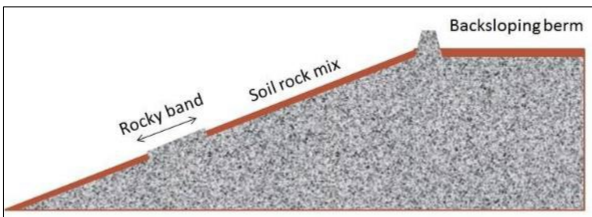
Figure 9-15: Closure Waste Dump Batter Design
