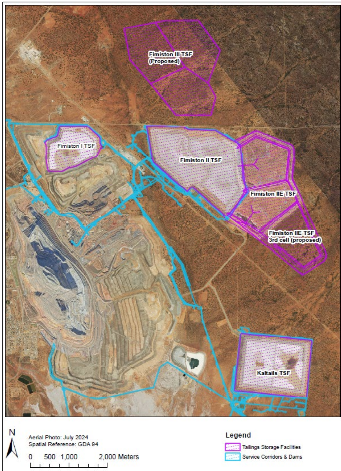
Figure 9-26: Fimiston Operational Area Tailings Storage Facilities
