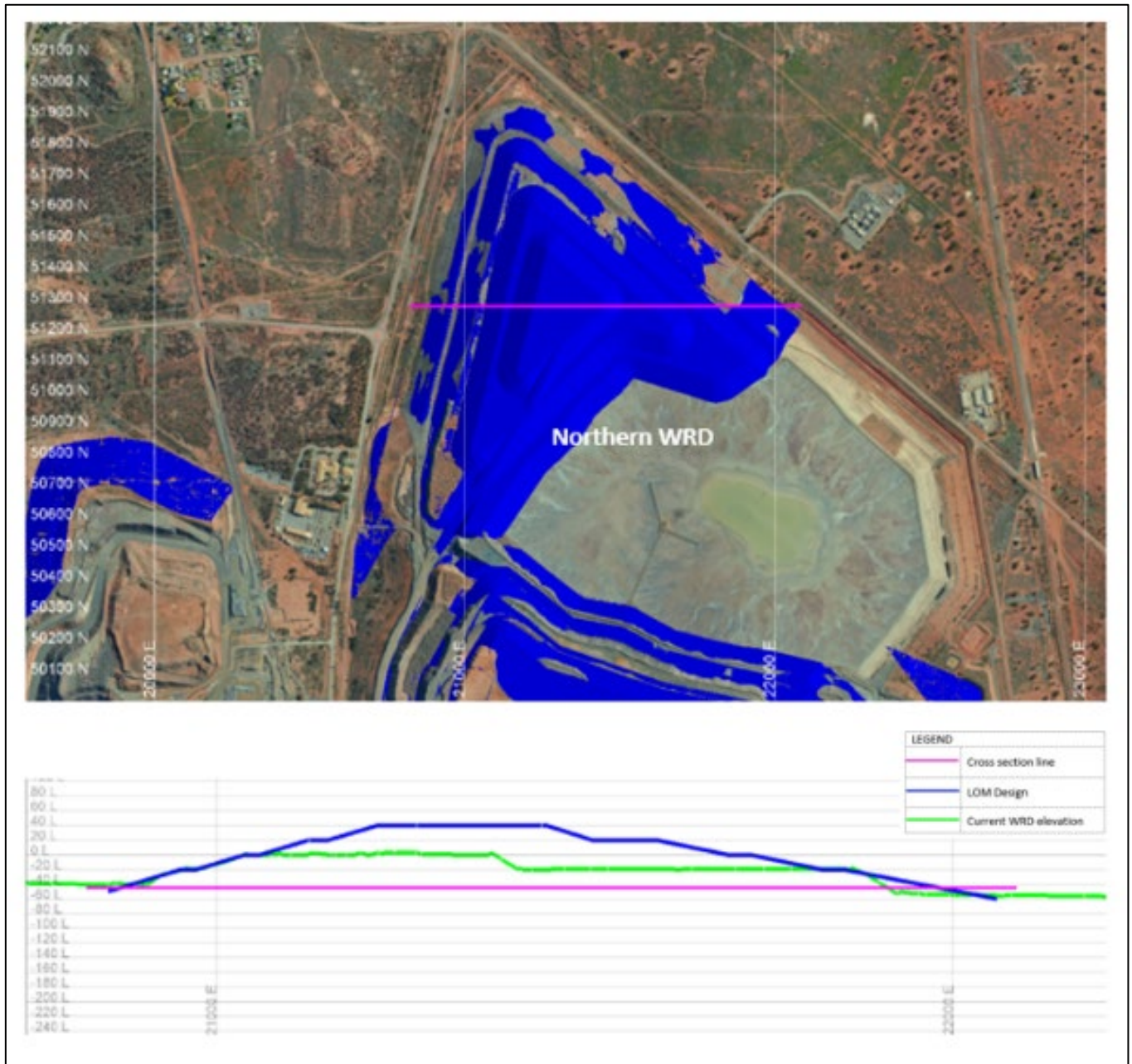
Figure 9-17: Fimiston Northern WRD Closure Design and Cross Section
