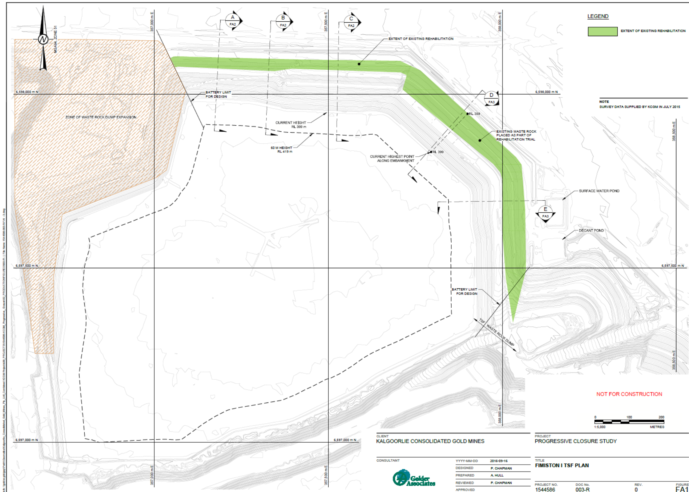
Figure 9-30: Fimiston I TSF Closure Design*
