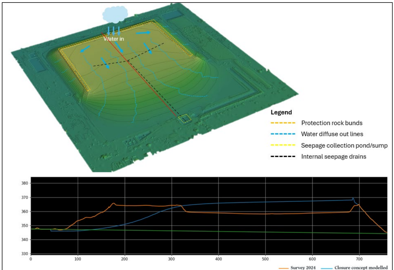
Figure 9-46 Proposed Gidji TSF Closure Design
