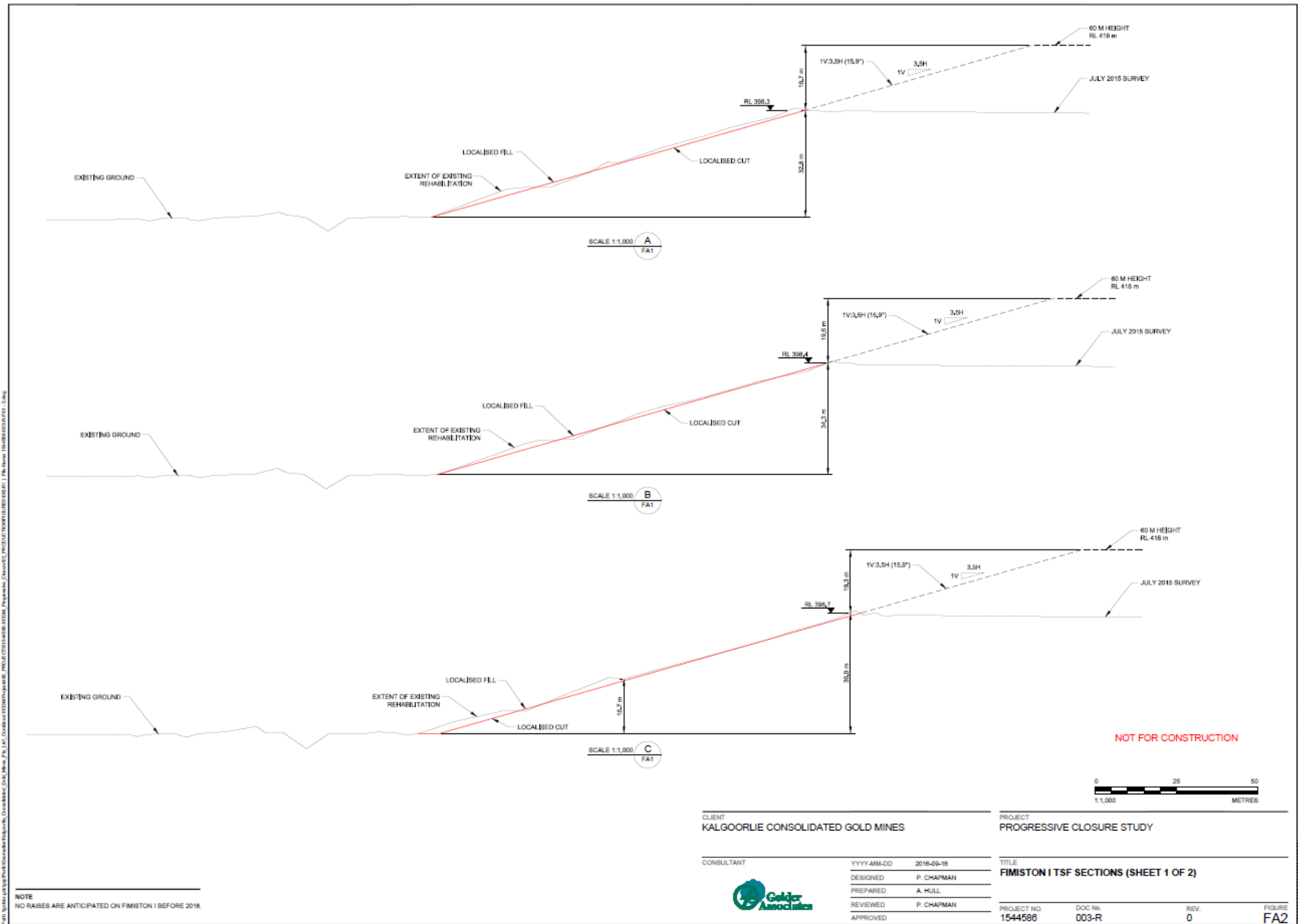
Figure 9-31: Fimiston I Closure Design Cross Sections
