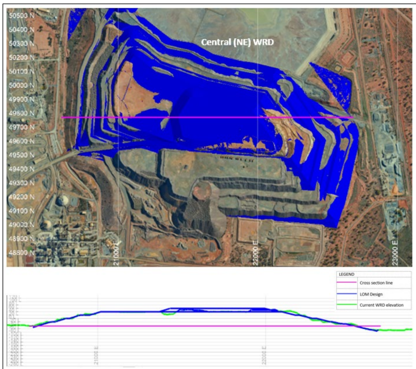
Figure 9-18: Fimiston Central WRD Closure Design and Cross Section
