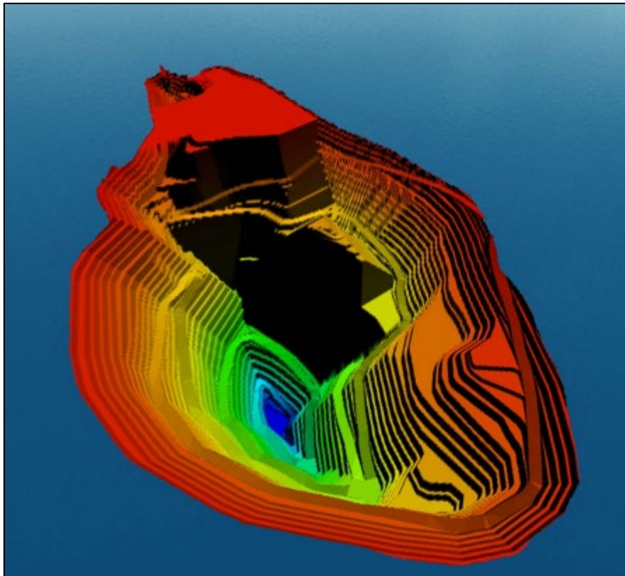
Figure 9-11: Planned backfill in the northern section of Fimiston Open Pit (schematic only)
