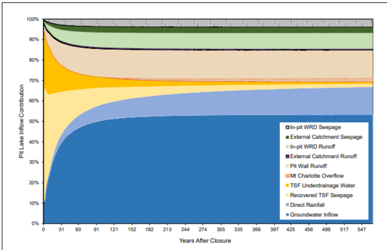
Figure 9-13: Pit lake water contributions over time
