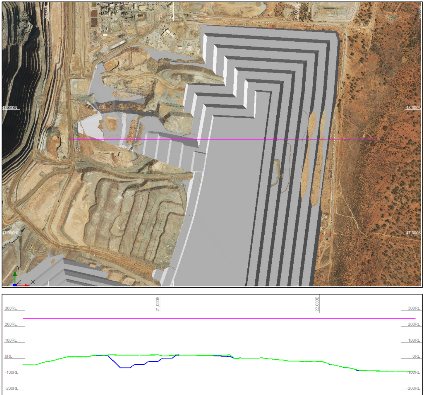
Figure 9-19: Fimiston Oroya WRD Closure Design and Cross Section
