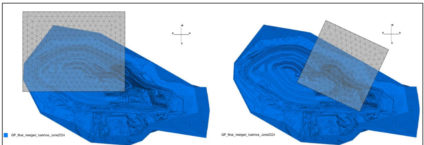
Figure 9-2: Ivanhoe cutback and Golden Pike Area geotechnical modelling of Fimiston Open Pit western wall.
