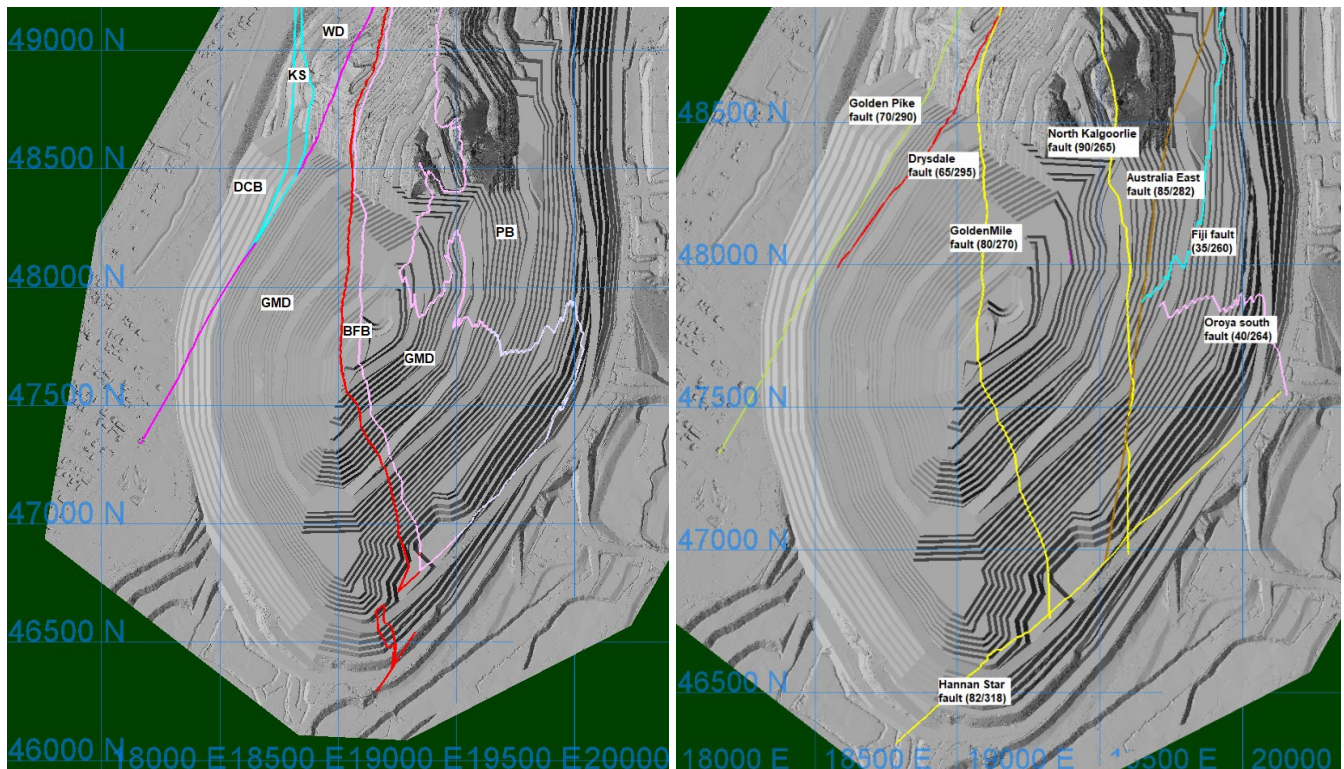
Figure 9-3: Ivanhoe cutback Project western wall showing major lithologies and structures modelled by (ITASCA 2025)
