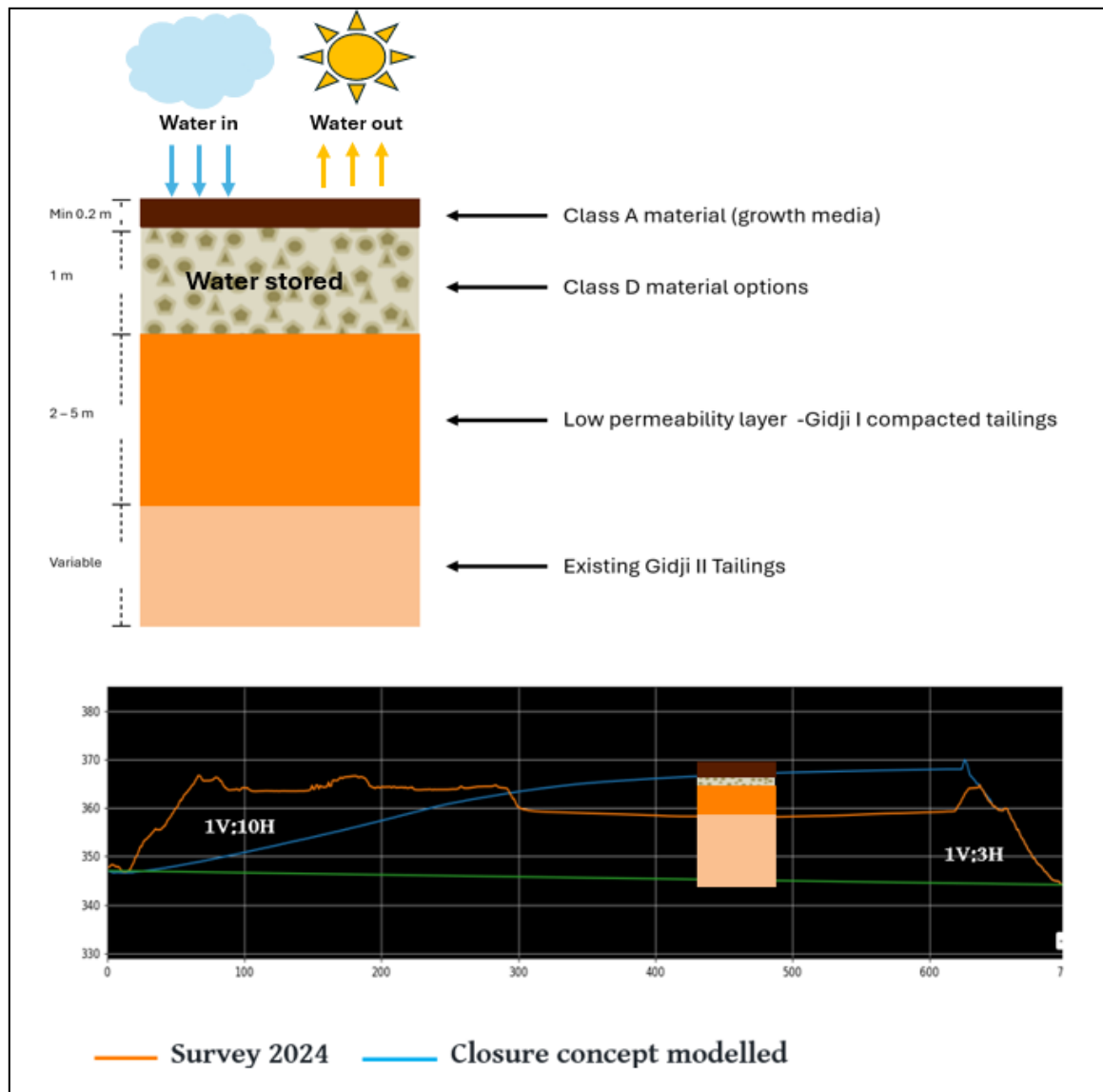
Figure 9-47 Proposed Gidji TSF cover design
