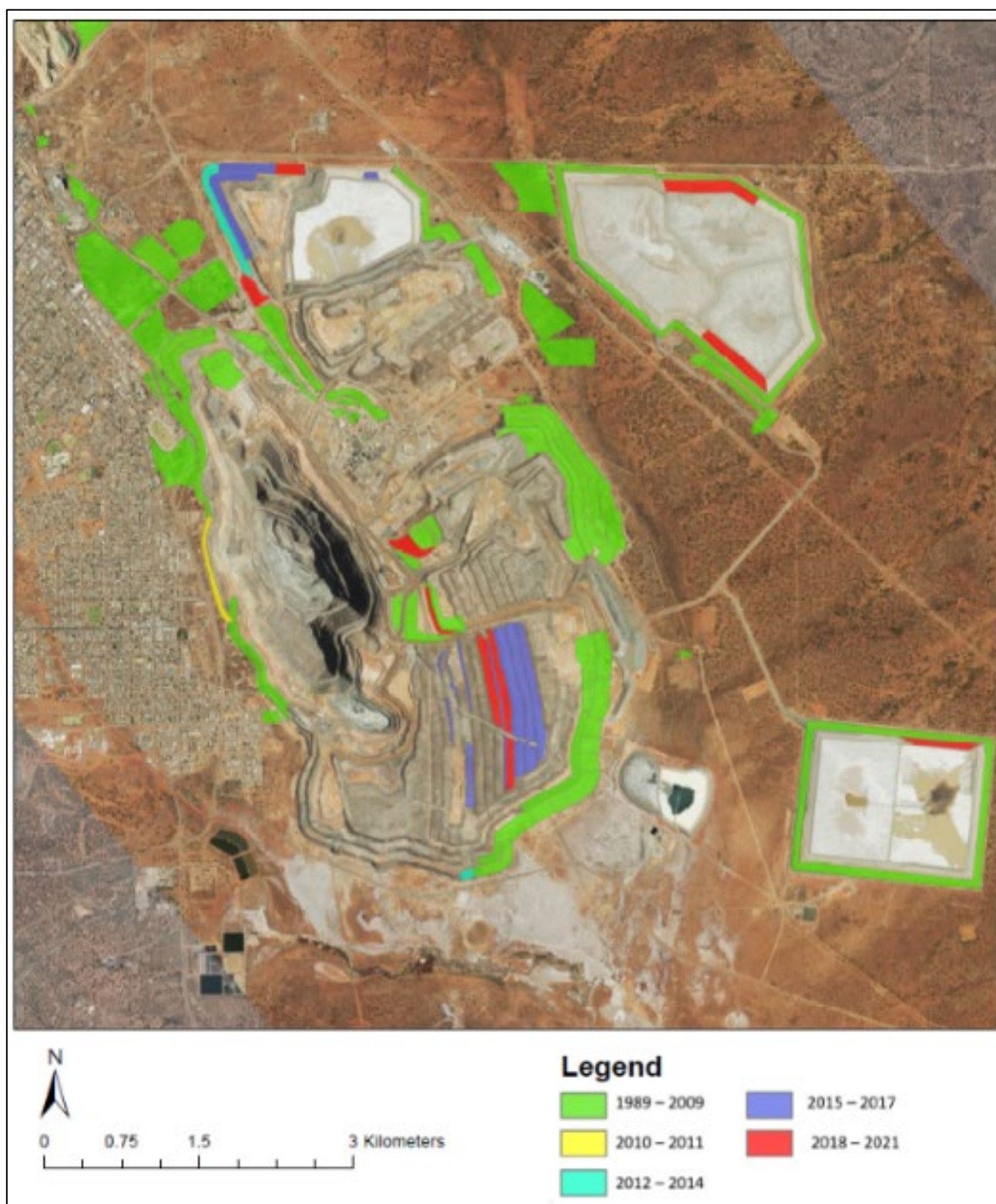
Figure 9-24: Progressive Rehabilitation at Fimiston WRDs 1995-2025 (to completed seeding)
