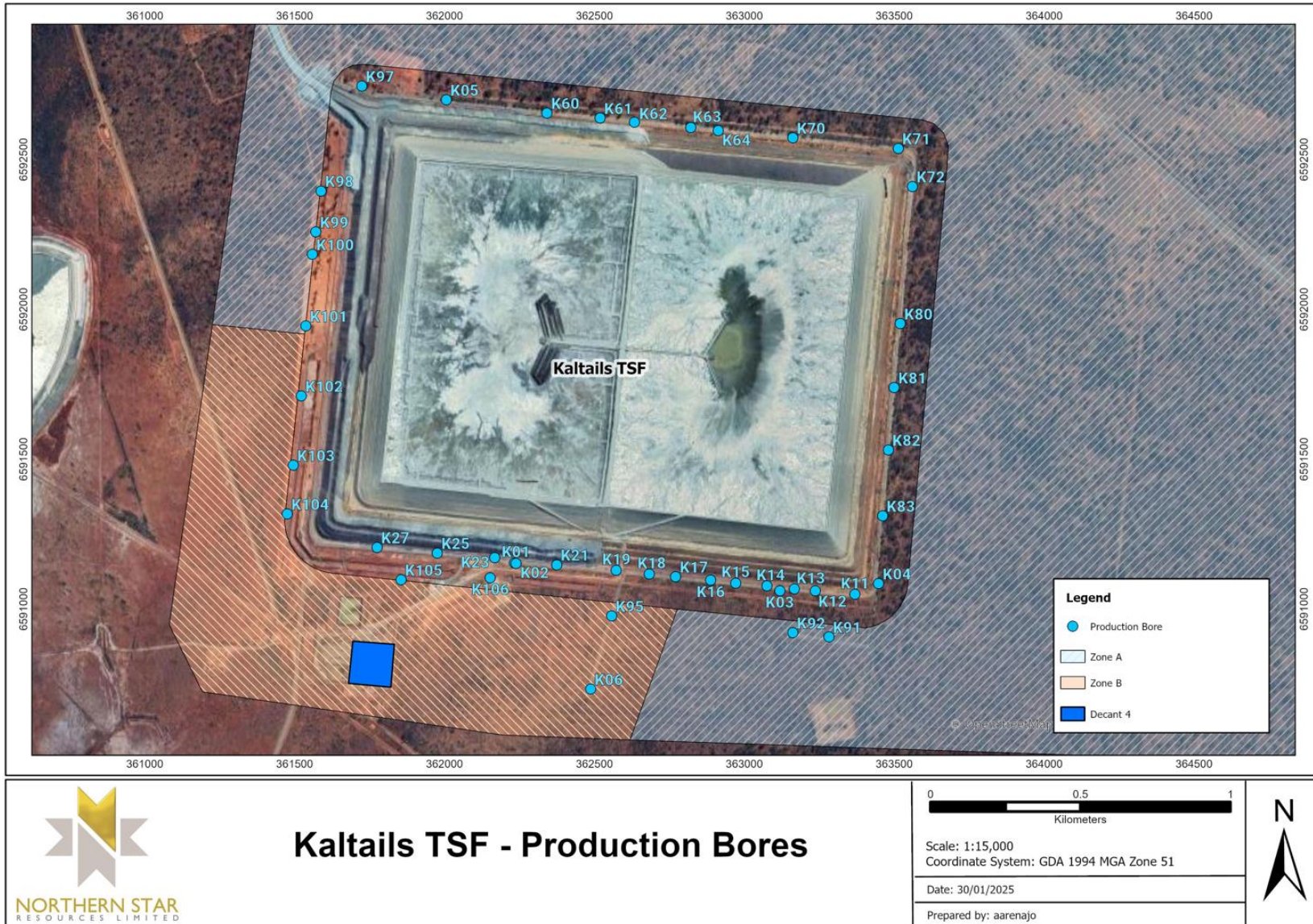
Figure 1. Location of Kaltails TSF Groundwater Production (Seepage Abstraction) Bores
